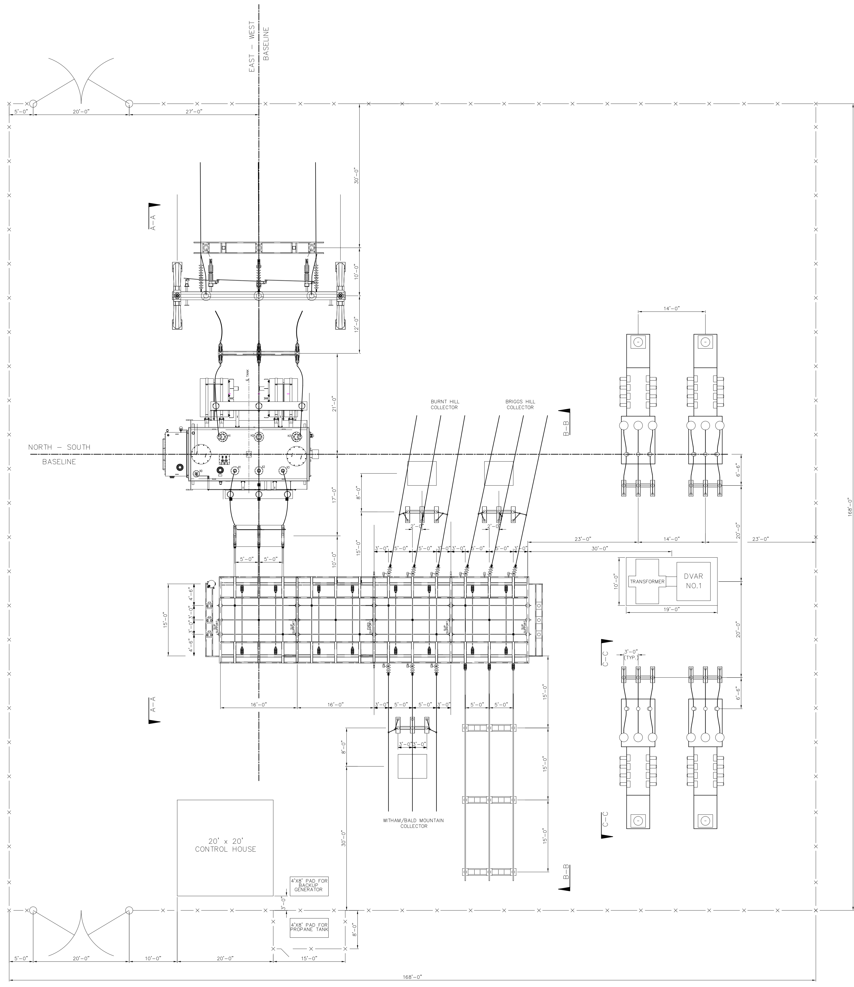
HIGHLAND WIND COLLECTOR SUBSTATION PLAN VIEW
